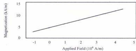
Fig. 1. Magnetization as a function of applied field. Note how the caption is centered in the column.
